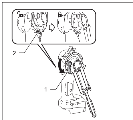
► 1. Lock lever 2. Lock-off switch
